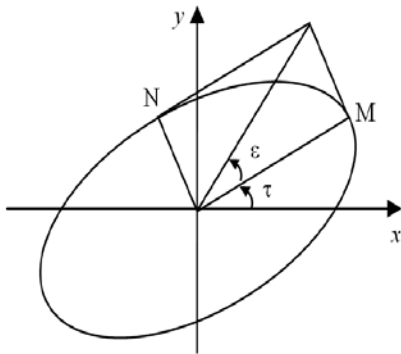
Figure 3. Polarization Parameters
