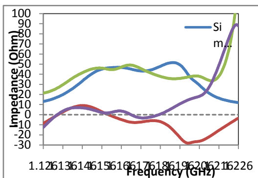
Figure 11. Simulated and measured input impedance ( Z_{in} ) plotted as a function of frequency.
