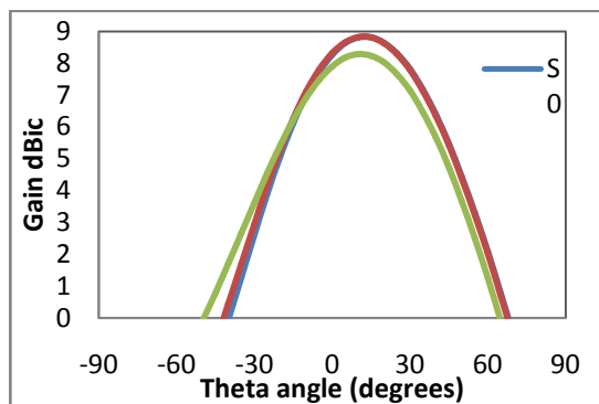
Figure 6. Simulation results showing the radiation pattern of the proposed antenna for various values of elements spacing (S)
