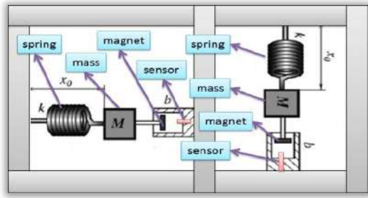
Figure 1. The design of the mechanical system
