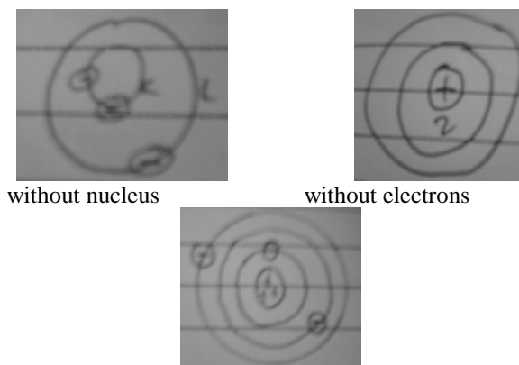
Less than 2 electrons in the first shell Figure 8. Misconception of Li atomic model
