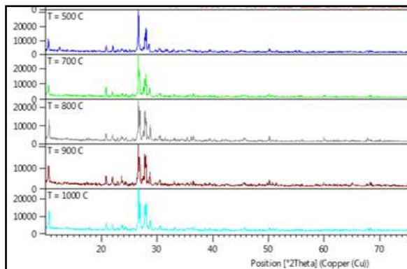
Fig 1. Spectra XRD of granite powder calcinated at 500 °C, 700 °C, 800 °C, 900 °C and 1000 °C.
