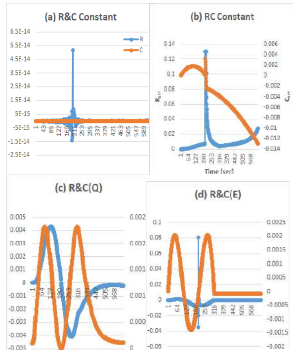
Figure 2. Error on the calculation of Rand C from the MPT to the case: (a) R&C Constant, (b) RC=Constant, (c) C linear Q, and (d) C linear ε.
