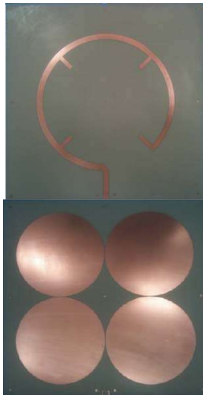
Figure 5. Photograph of fabricated proposed antenna: (a) synchronous feed, and (b) 2x2 circular radiators.
