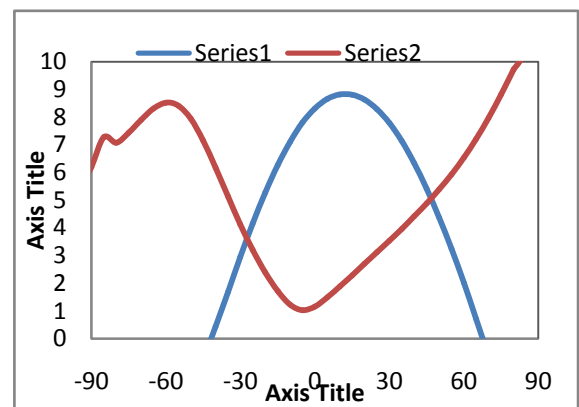
Figure 14. Array antenna characteristics in the theta plane ( x - z plane) at f = 1.27 GHz: (a) gain versus theta angle, and (b) axial ratio versus theta angle.
