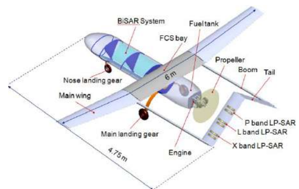
Figure 1. Illustration of the bi-static SAR
