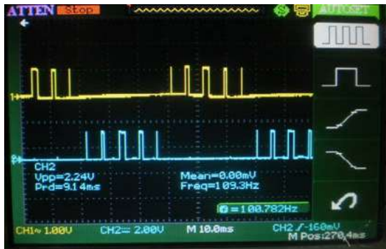
Figure 4. PWM pulse oscilloscope photograph of real measurements
