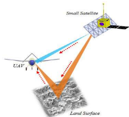
Figure 1. Illustration of the bi-static SAR
