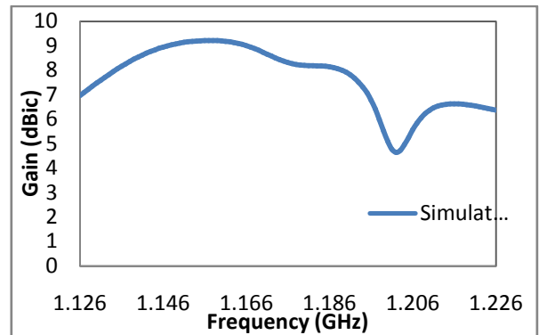
Figure 13. Simulated and measured gain ( G ) vs. frequency at \theta = 0^\circ .
