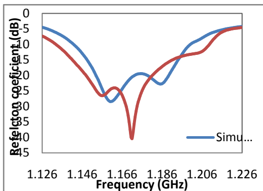
Figure 10. Simulated and measured reflection coefficient vs. frequency
