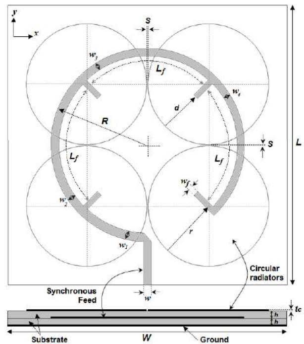
Figure 4. Configuration of sub array circular synchronous feed
