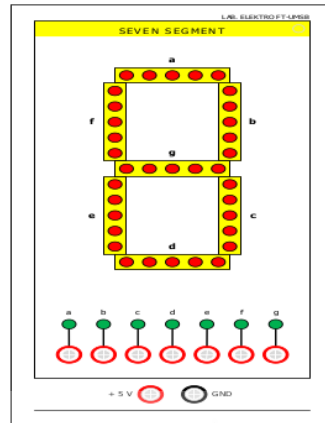
Gambar 3.13. Layout seven segment modul
