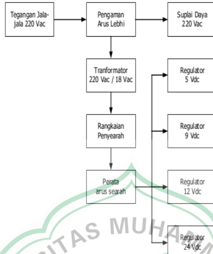
Gambar 3.3. Blok diagram power suplai
