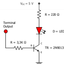
Gambar 3.8. Rangkaian driver LED
