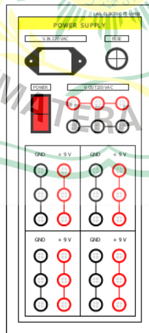
Gambar 3.4. Layout power supply modul
