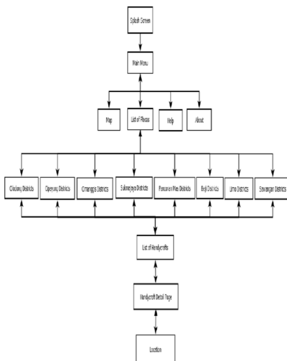
Figure 3.2 Navigation Structure
