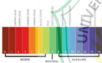
Gambar 1 Skala Derajat Keasaman (pH)
