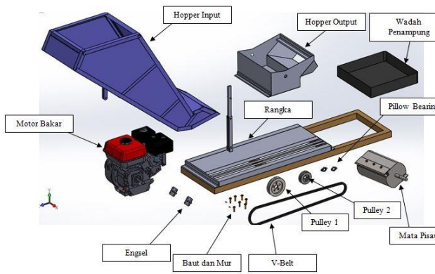
Gambar 2. Explode View
